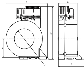
RCMB 30... + CTBC60(P)
